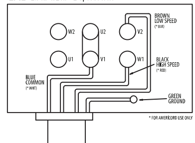
EME - 2.5 HP & 2 HP - 2-Speed Motor
