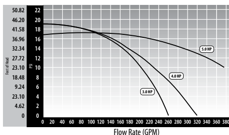
PRESSURE VERSUS FLOW RATE
